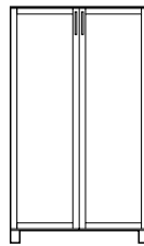
Cabinet 80w x 40d x 137h Art No 010026- Only in oiled oak and pure white
